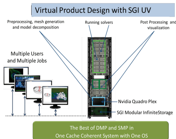
Fig. 3: SGI UV CAE Workflow
