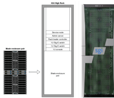
Fig. 2: SGI ICE X Cluster with Blade Enclosure
