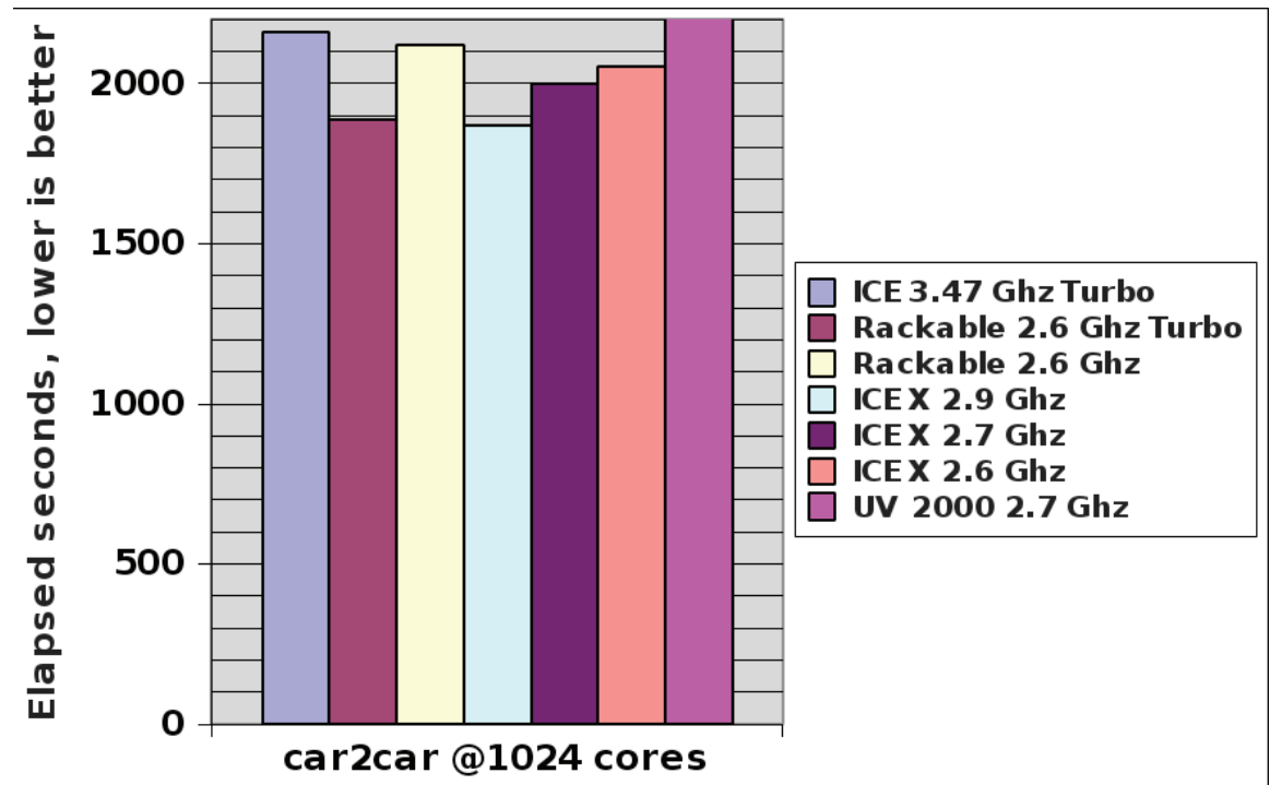
Figure 11: Elapsed time comparisons between platforms, car2car
