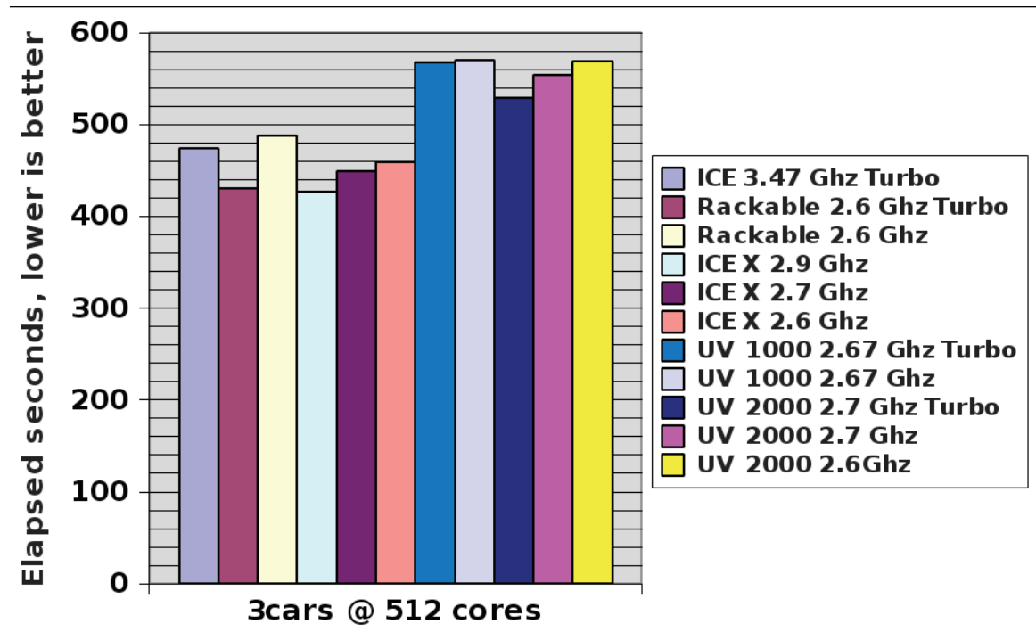
Figure 10: Elapsed time comparisons between platforms, 3 vehicle collision
