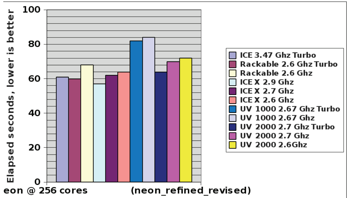
Figure 9: Elapsed time comparisons between platforms, neon refined revised
