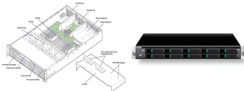
Fig. 1: Overhead View of SGI Rackable Server with the Top Cover Removed and Actual Server
