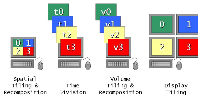
Figure 2.12: Example tiling techniques for scaling graphics performance.
